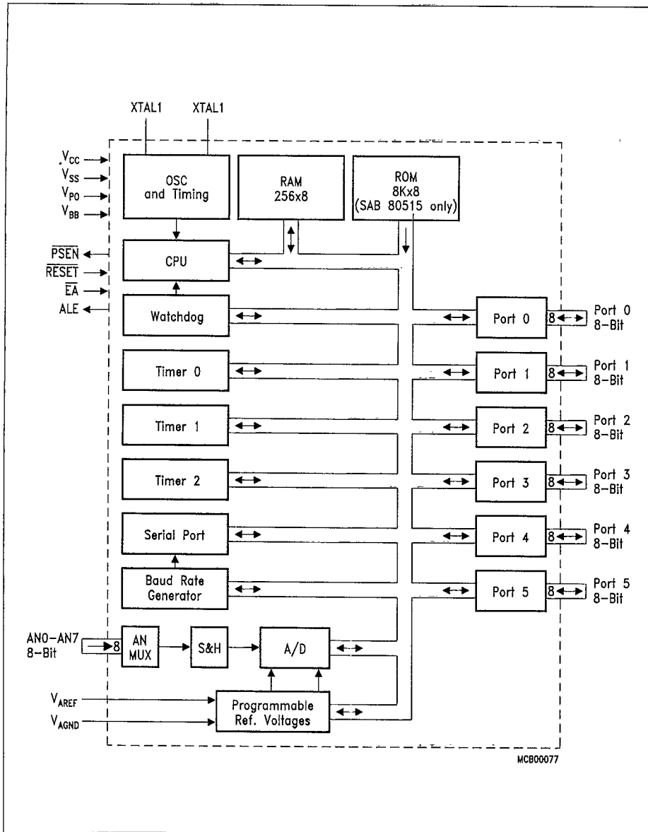
Figure 1 Block Diagram
