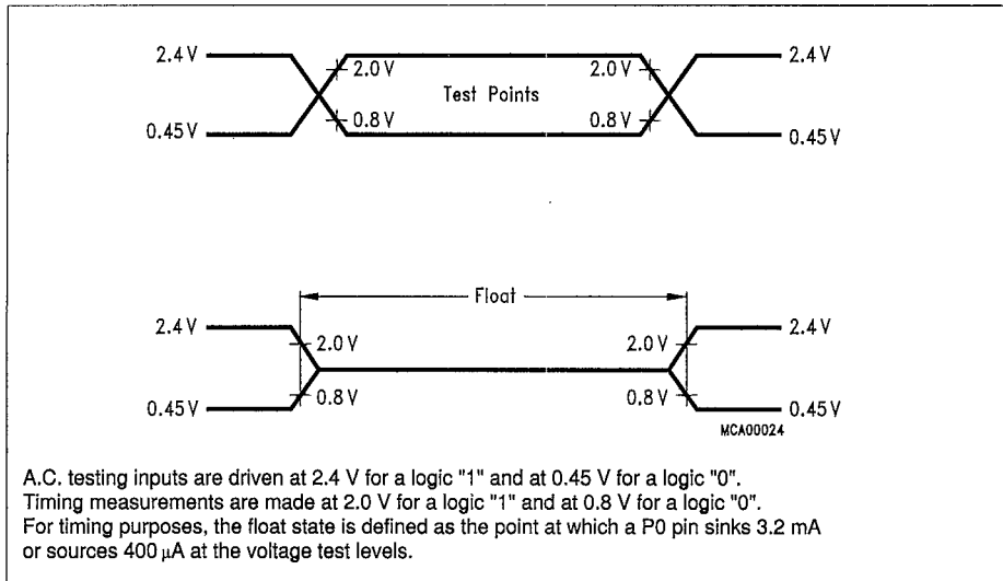
A.C. Testing Input, Output, Float Waveforms
