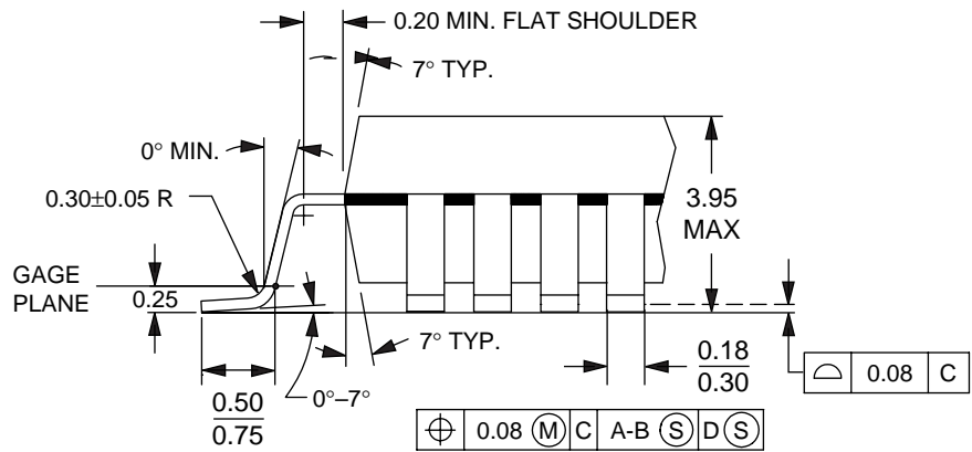
DETAIL X
