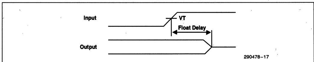
Figure 16. Float Delay
