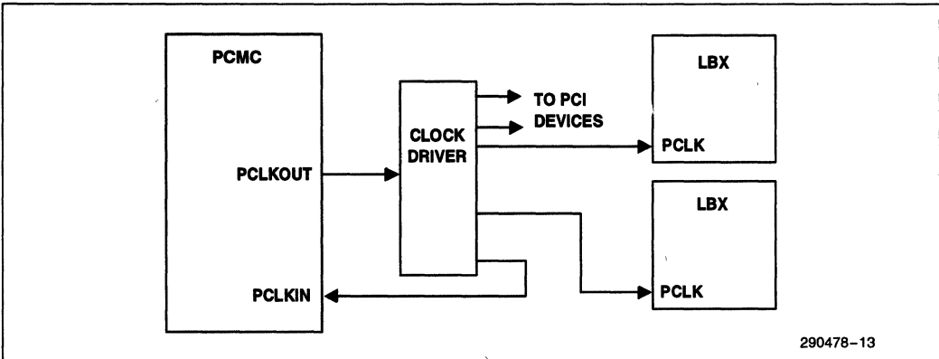
Figure 12. Clock Considerations
