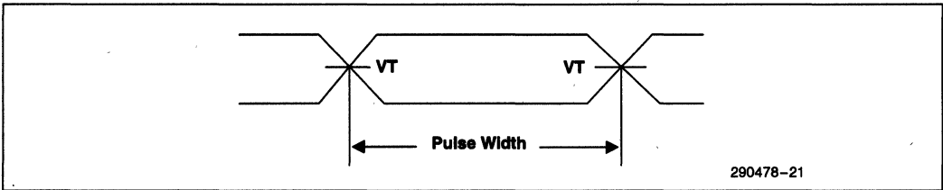
Figure 20. Pulse Width
