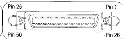
Figure 4 Device Connector
