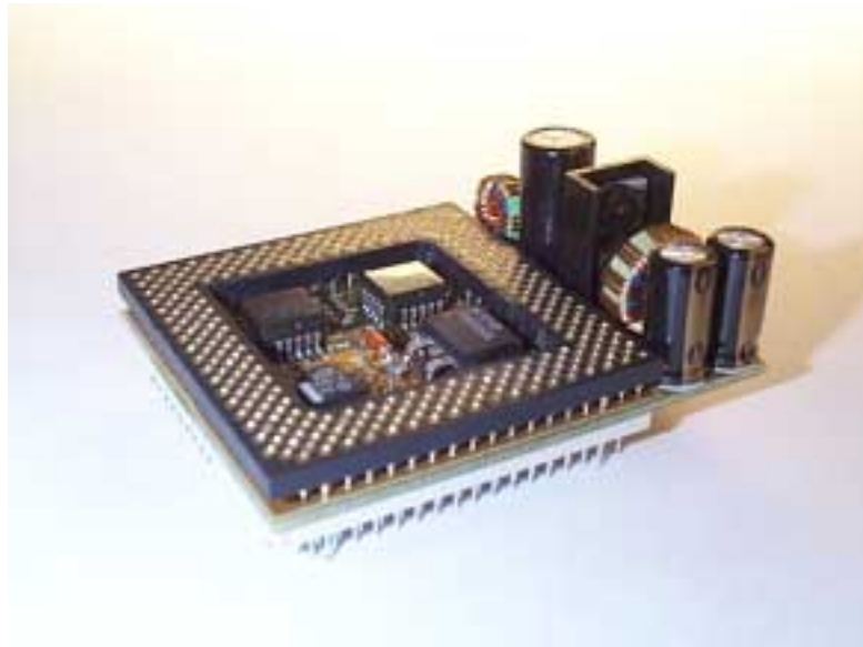
Figure 1. The PL-K6-III/98
