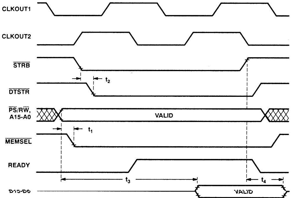
Figure 15. Interface Timing of the WS57C64F-12 to the TMS320C2x
