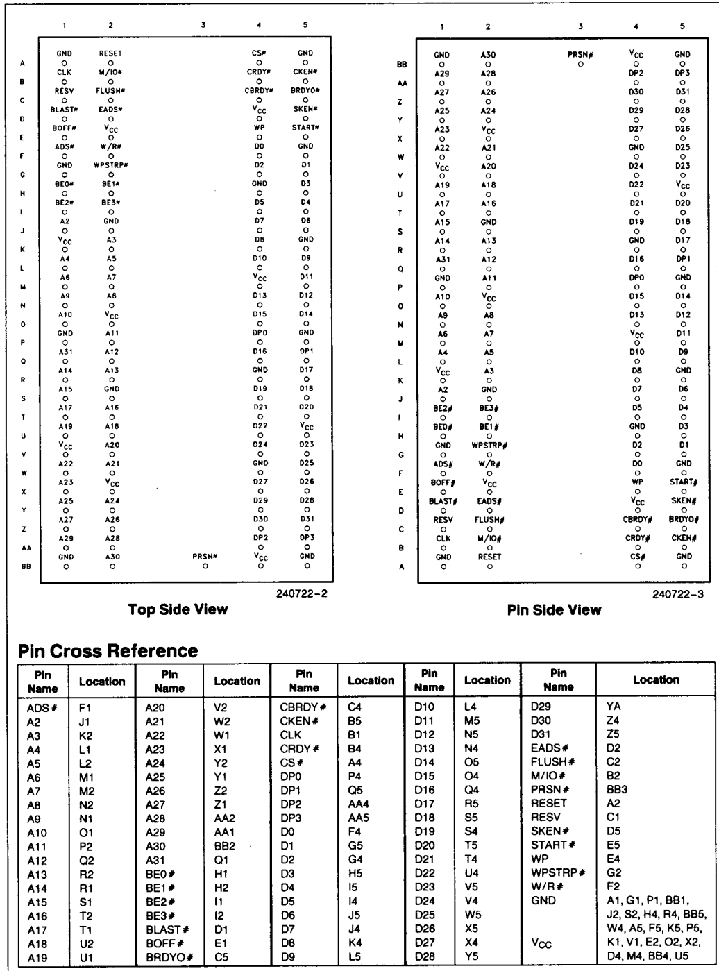
Figure 0.2. 485Turbocache Module 64k/128k Pin Configuration
