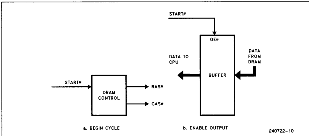
Figure 3.1. Using START# in DRAM Control
