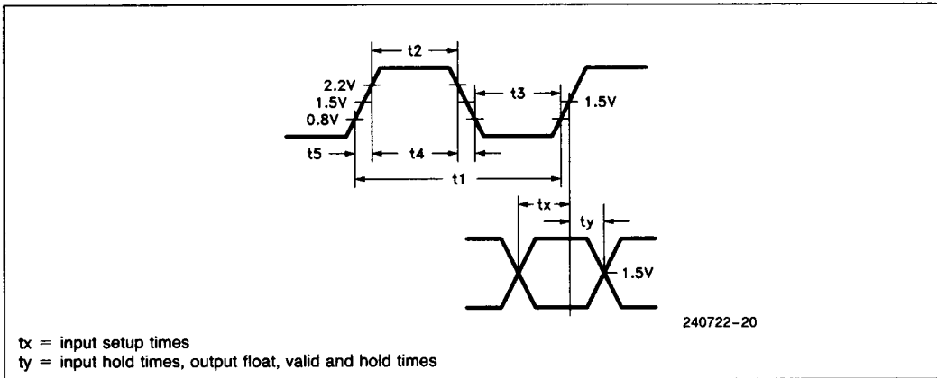
Figure 9.1. CLK Waveforms
