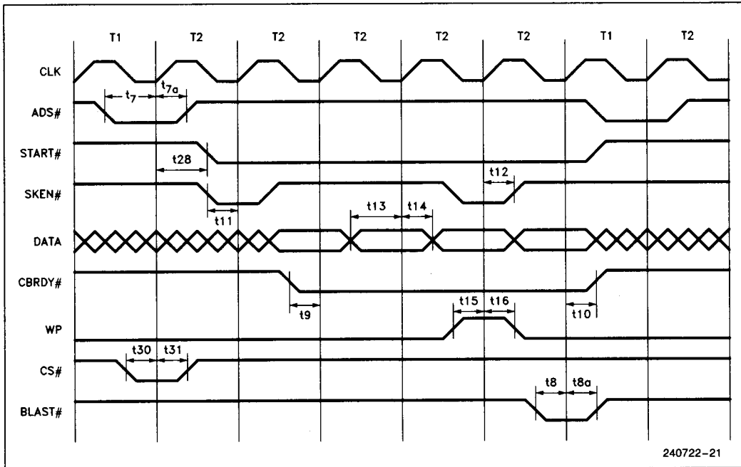
Figure 9.2. Write Protected Read Miss
