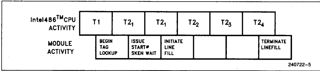
Figure 1.2. Normal Read Miss Cycle
