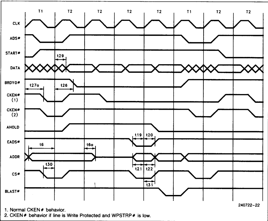
Figure 9.3. Read Hit Cycle and Write Cycle with Invalidation
