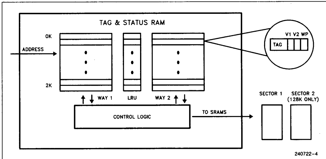
Figure 1.1. 82485 Cache Controller 2-723
