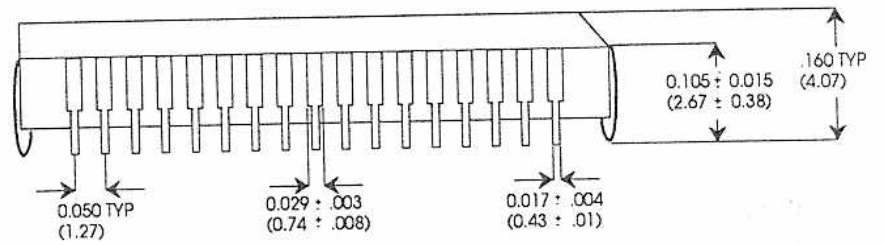
PLCC Package
