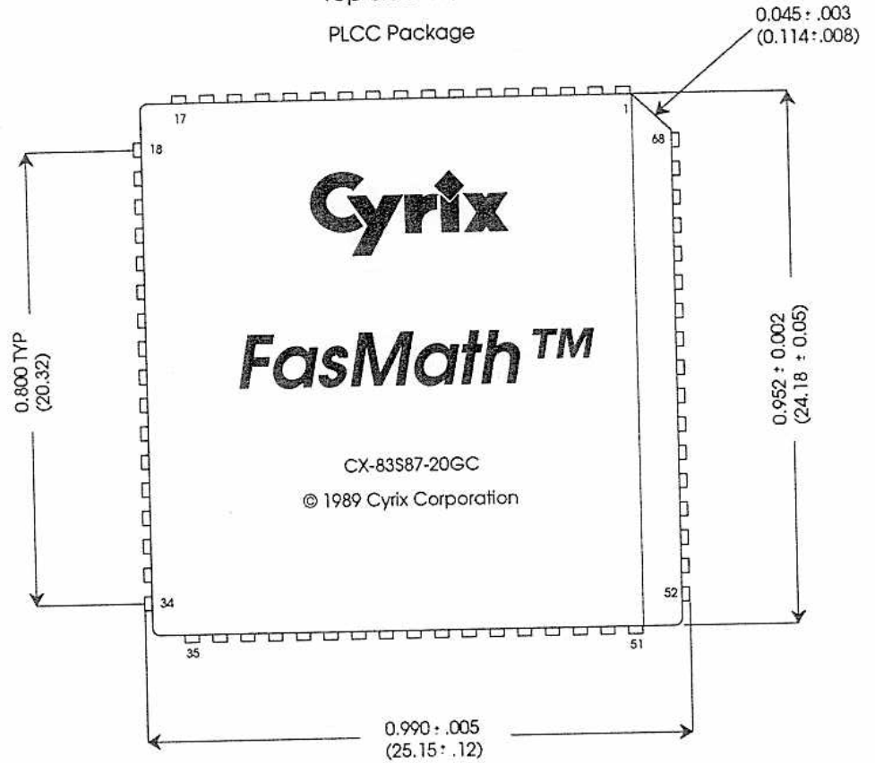
PLCC Package
