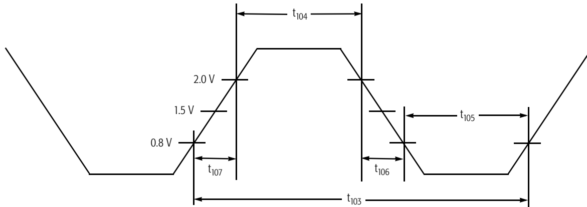
Figure 110. TCK Waveform
